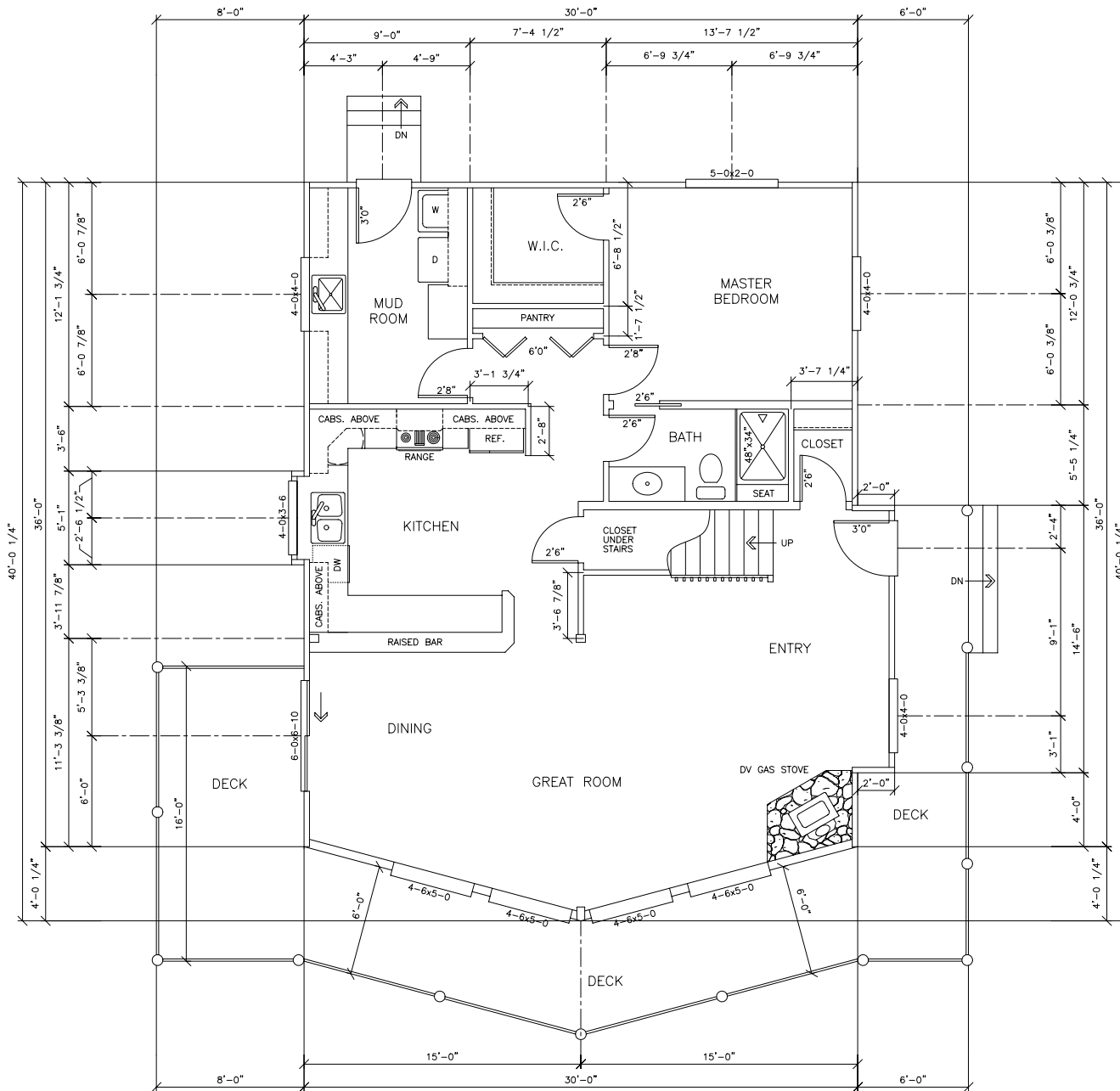
© Cedar Homes PO Box 8265 Fort Collins, CO 80526 1 (800) 98CEDAR www.CedarTimbers.com BEAR TRAP STUDY PLAN MAIN LEVEL 1,173 SF
