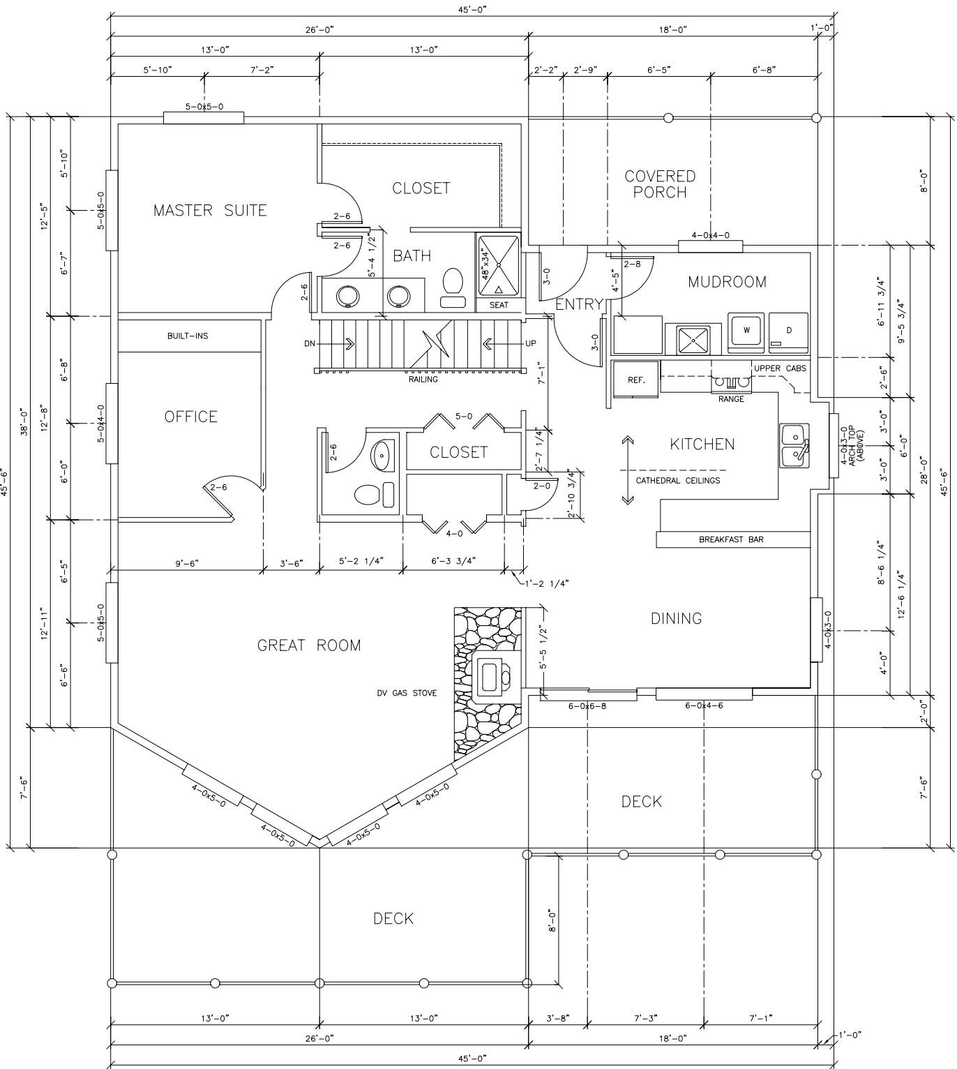
© Cedar Homes PO Box 8265 Fort Collins, CO 80526 1 (800) 98CEDAR www.CedarTimbers.com LAKEVIEW STUDY PLAN MAIN LEVEL 1,596 SF
