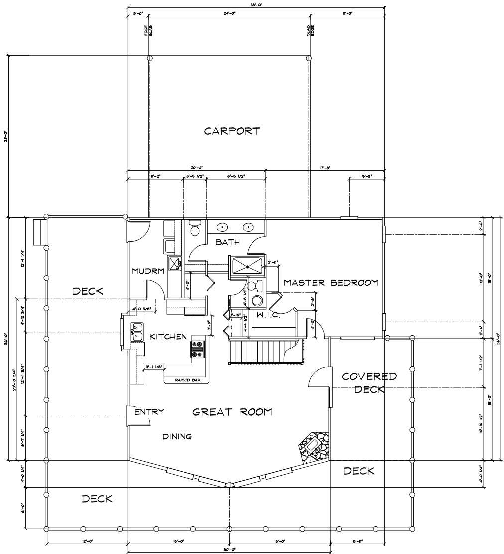
© Cedar Homes 1290 SF 1 GARAGE www.CedarHomes.com BRECKENRIDGE STUDY PLAN MAIN FLOOR PLAN 1290 SF
