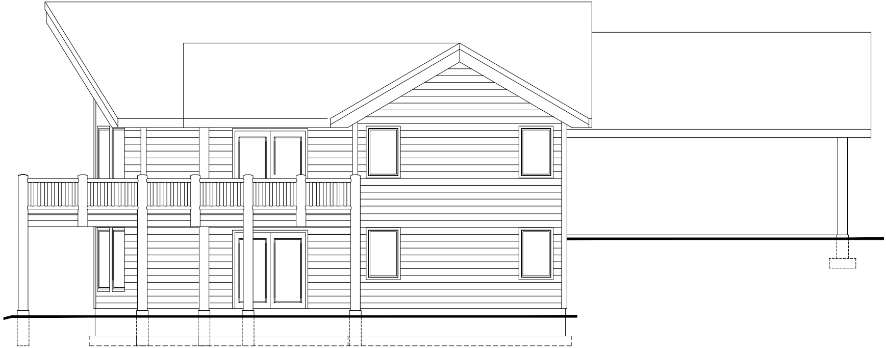
© Cedar Homes PO Box 276218 Fort Collins, CO 80527 1 (800) 98CEDAR www.CedarHomes.com BRECKENRIDGE STUDY PLAN ELEVATION
