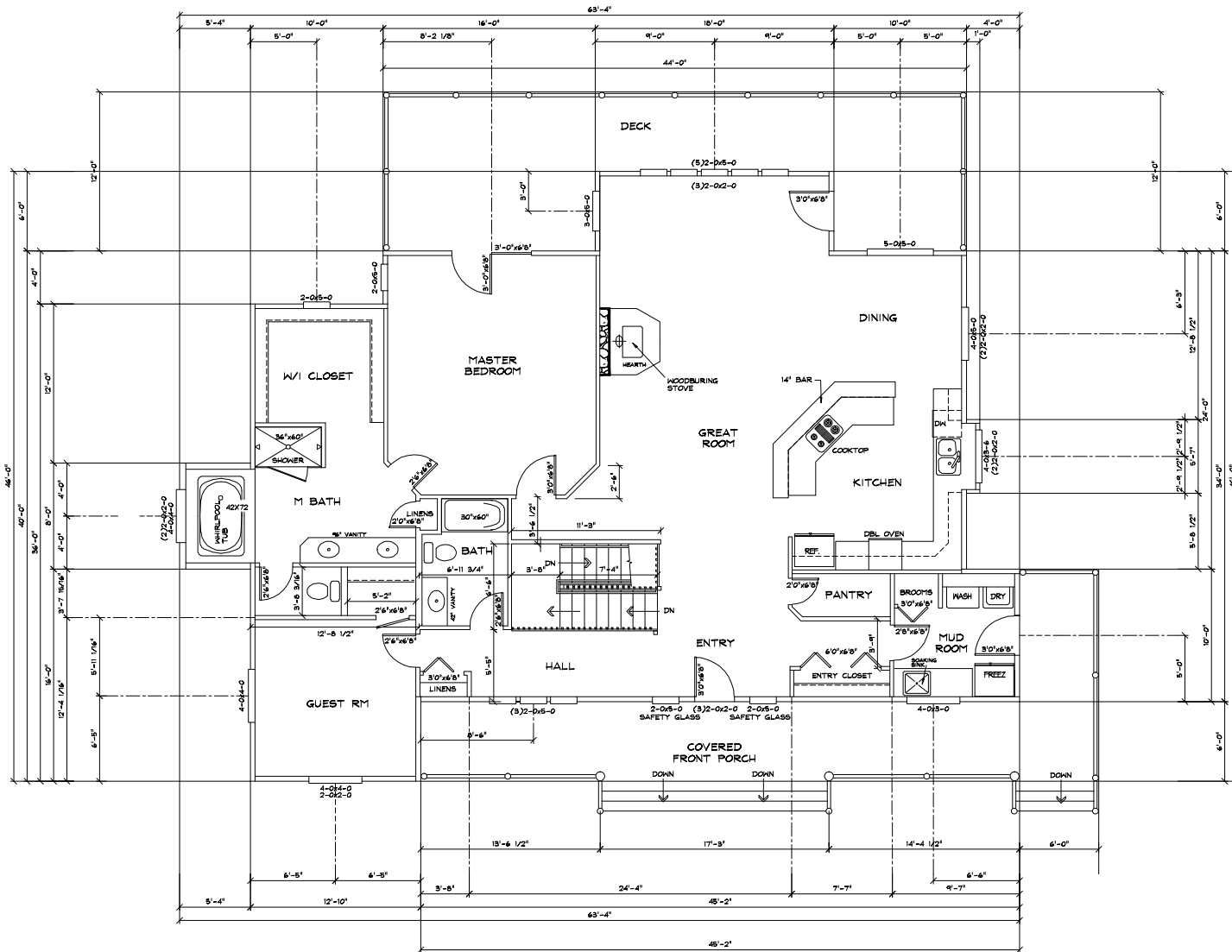
© Cedar Homes 10100 20th St Fort Collins, CO 80501 1 970 226 2222 www.cedarhomes.com CIMARRON STUDY PLAN MAIN FLOOR PLAN 2070 SF
