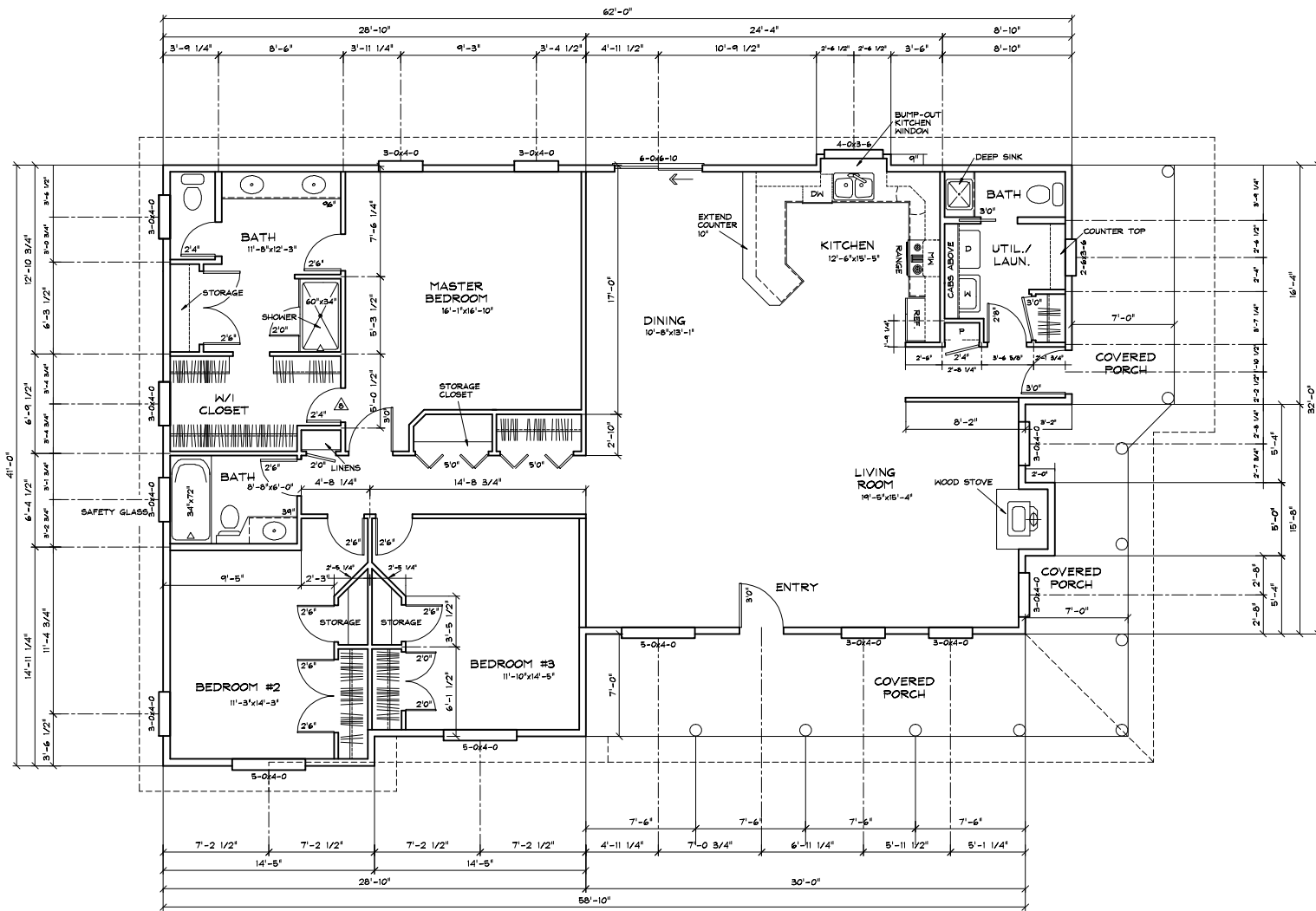
© Cedar Homes 701 W. 22nd St. Fort Collins, CO 80521 1 (970) 223-2242 www.CedarHomes.com PRAIRIE RANCH STUDY PLAN MAIN FLOOR PLAN 2175 SF
